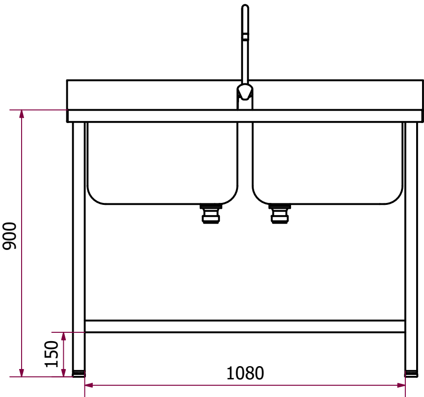
VISTA FRONTAL
