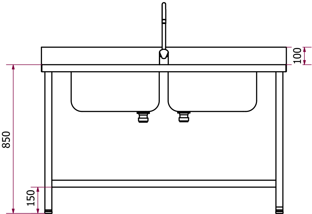
VISTA FRONTAL
