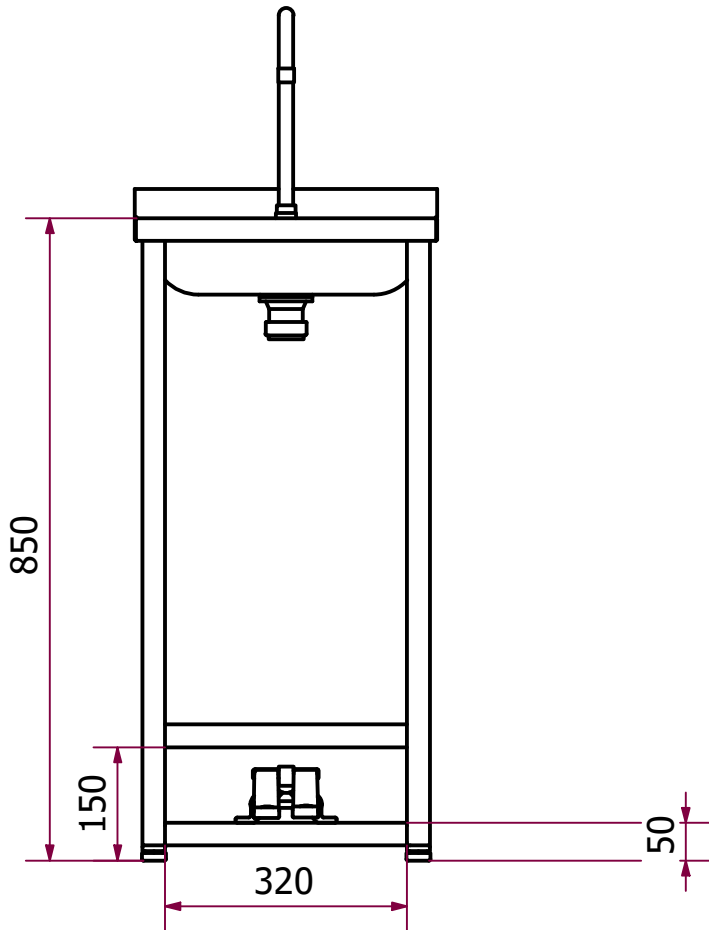
VISTA FRONTAL
