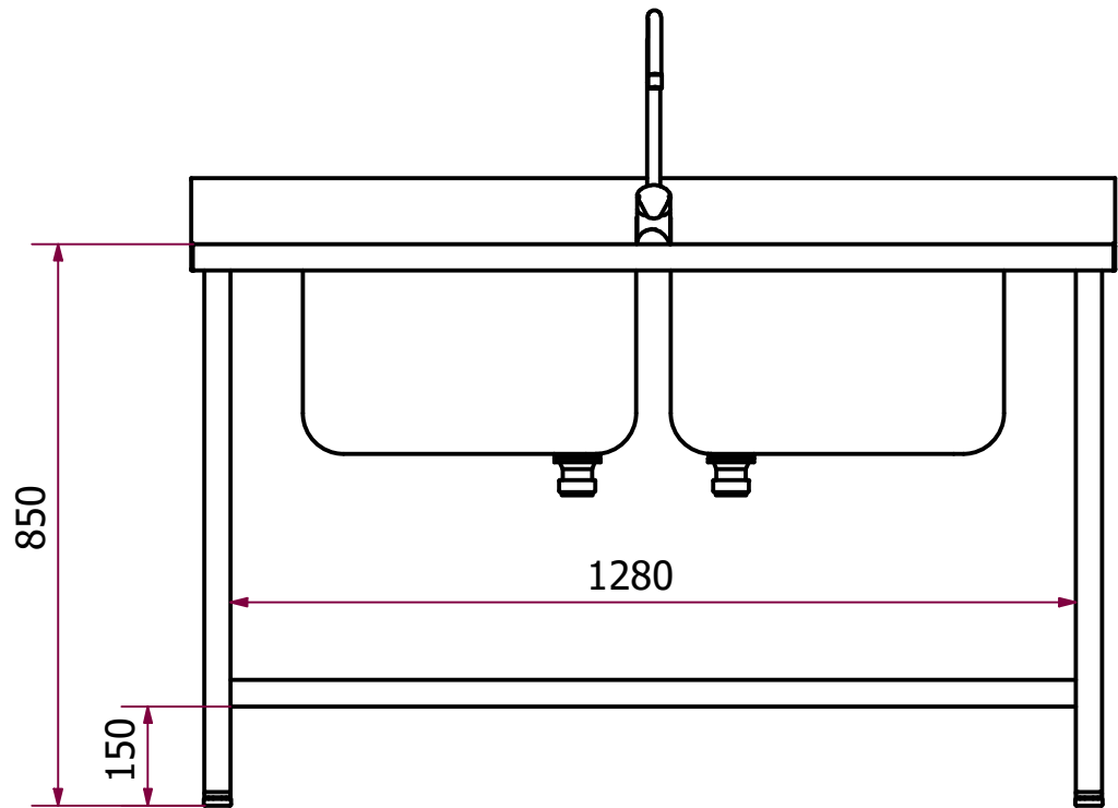
VISTA FRONTAL
