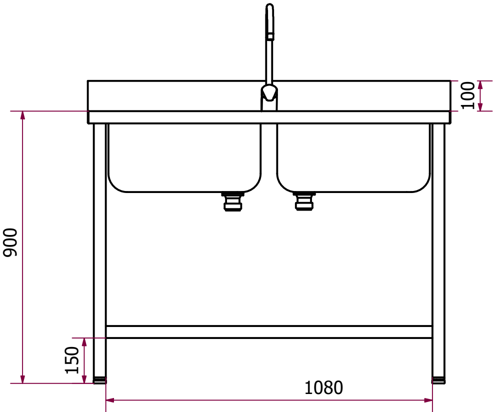
VISTA FRONTAL
